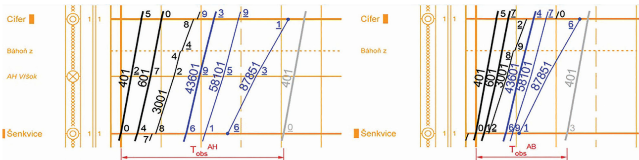
a) trains sequence under automatic block signal ABS
