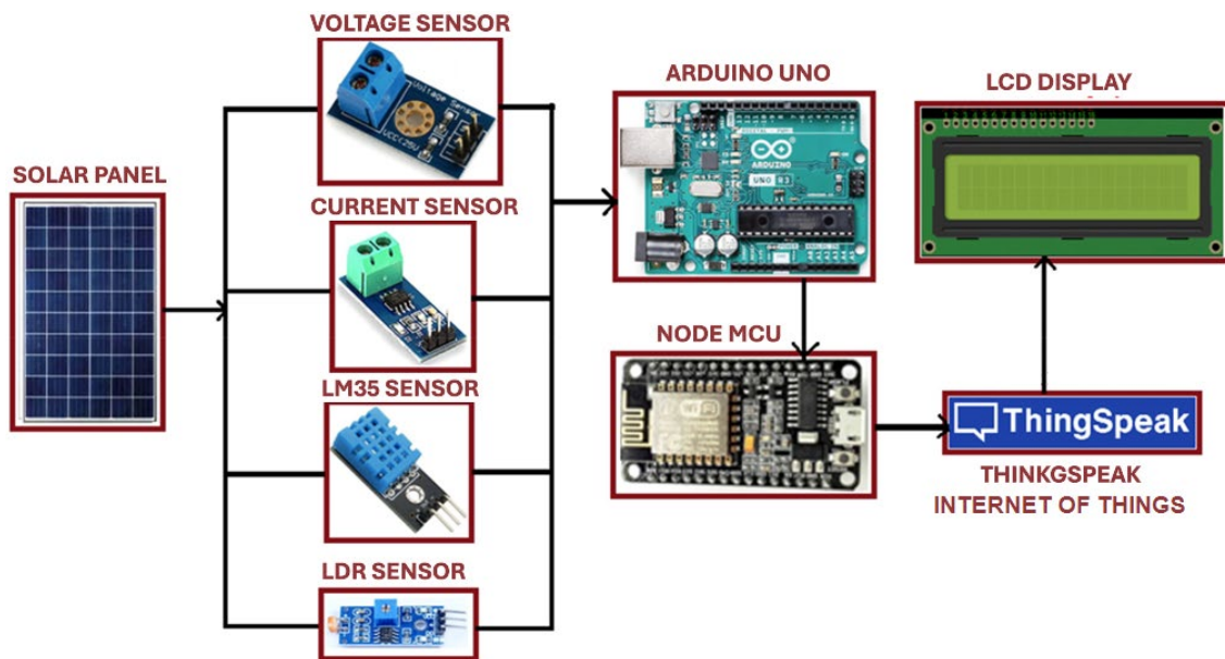
Figure 2 The proposed solar power monitoring system [6]
